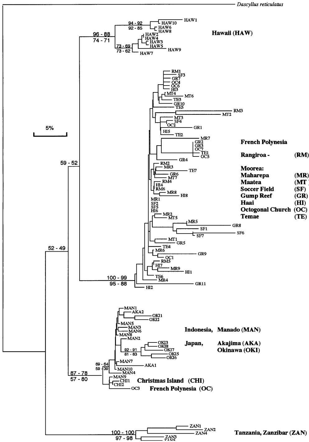
Fig. 2 Dascyllus trimaculatus phylogenetic relationships using the neighbor-joining method (unrooted tree). The right panel indicates a list of abbreviations used in the tree and in Fig. 1. Numbers above the major nodes indicate bootstrap support using the neighbor-joining method with equal weights for transitions and transversions (first number), and when transversions are weighted three times as much as transitions (second number). Numbers below the major nodes correspond to bootstrap support using the maximum parsimony method with equal weights and 3:1 weights for transversions and transitions. In all cases, 500 bootstrap replicates were used. Other numbers indicate bootstrap support using the neighbor-joining method, with equal weights for transitions and transversions (only values above 85% are shown)
