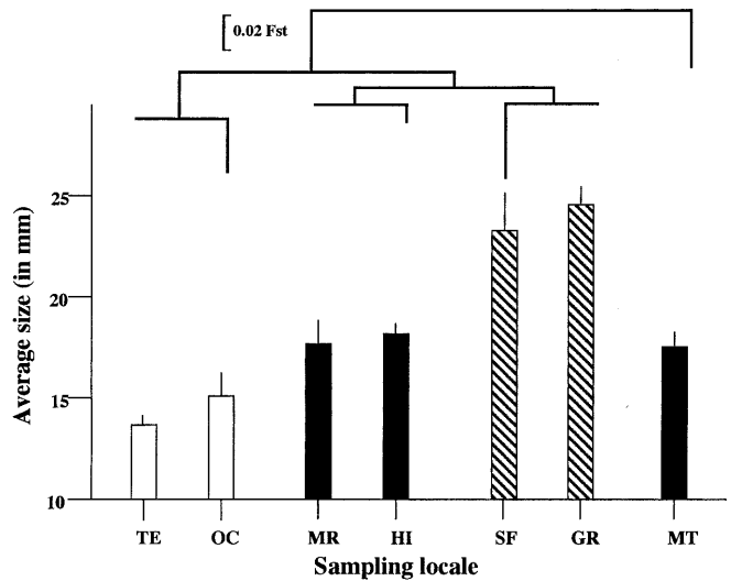
Fig. 3 Dascyllus trimaculatus relationships between average size per locality and F_{st} distances between Moorea populations. Histograms represent the average size (total length) of the fish collected (white bars small sizes; black bars medium sizes; hatched bars large sizes). Sizes are given in millimeters; bars represent standard error. Sampling locality abbreviations and geographic locations are given in Fig. 1. A tree based on F_{st} distances (neighbor-joining method) represents the relationships between locales
